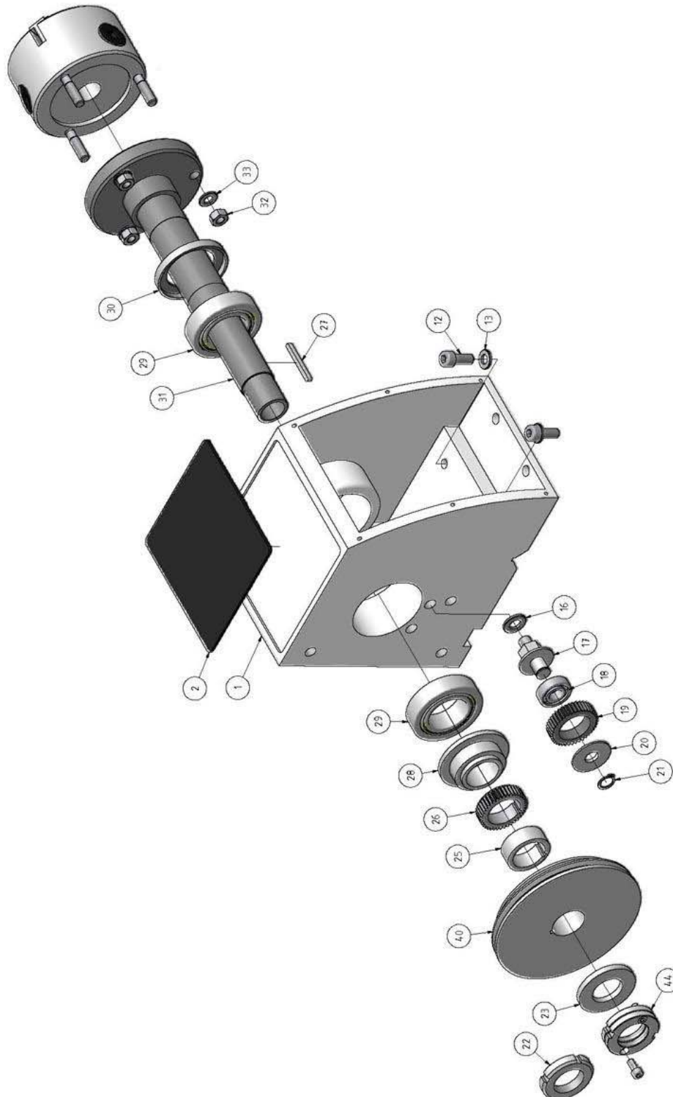
1-8: Spindelstock - Headstock
