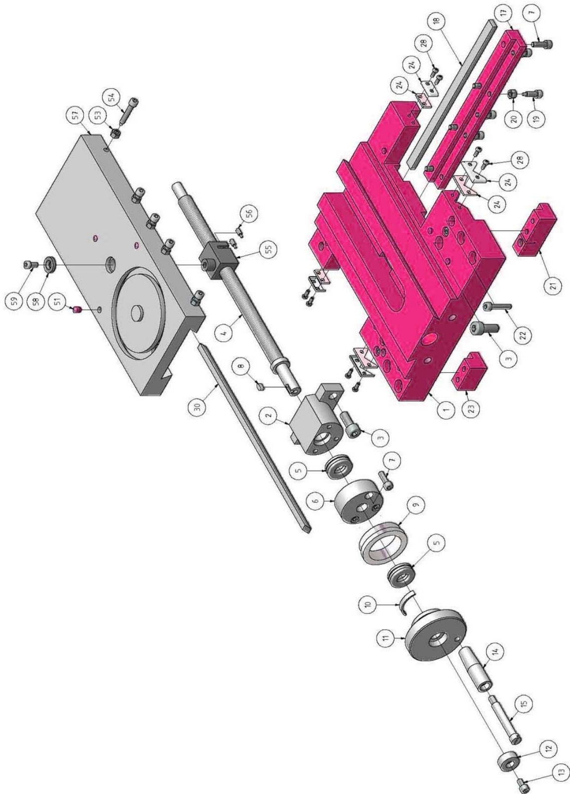
1-2: Planschlitten - Cross slide
